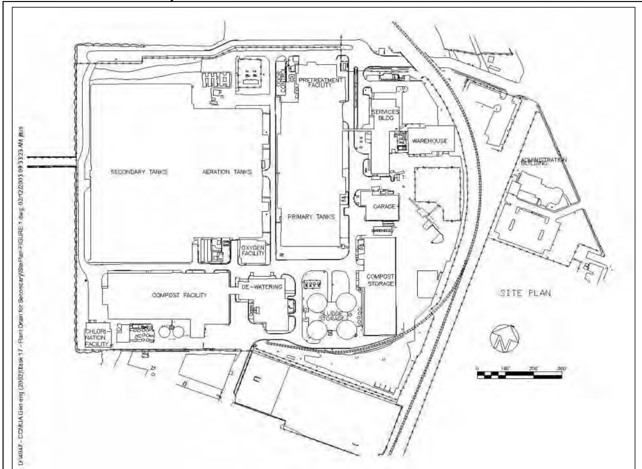
Figure 2-2 – Plan View of CCMUA Delaware Water Pollution Control Facility #1
